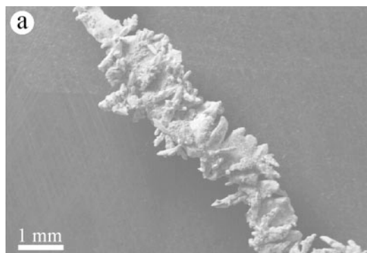
FIG. 2. SEM images of (a) a palladian gold thread and (b) an arborescent palladian gold aggregate from Serra Pelada.
